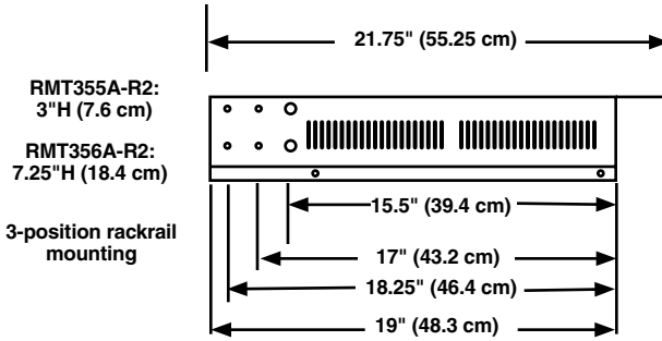
Figure 1. Side view.
