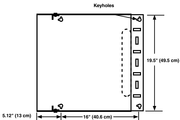
Figure 4. Top view with cover.
